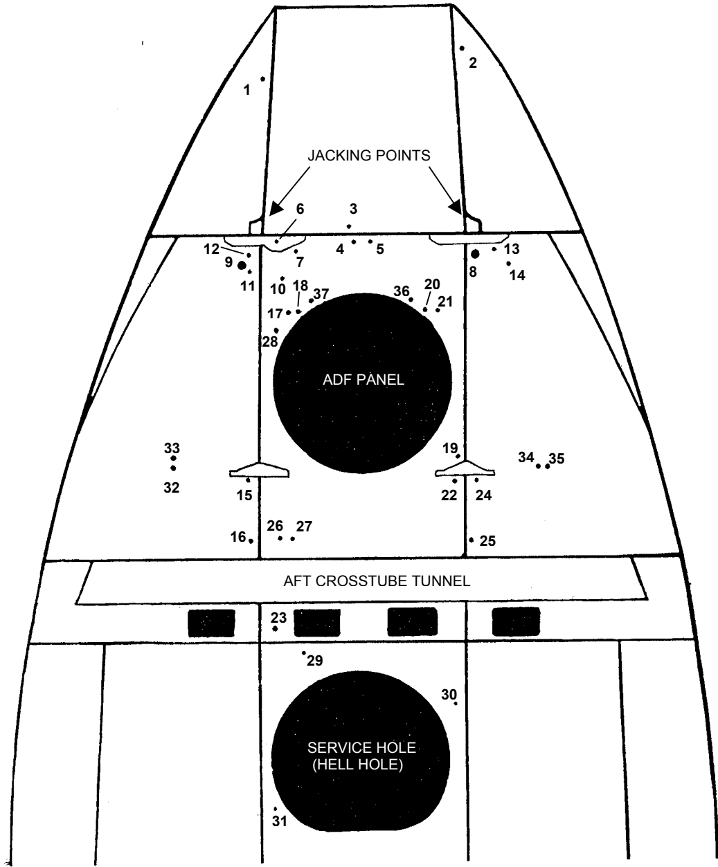
Figure 2 Model 412, 412EP & 412CF Belly (Looking Up)
