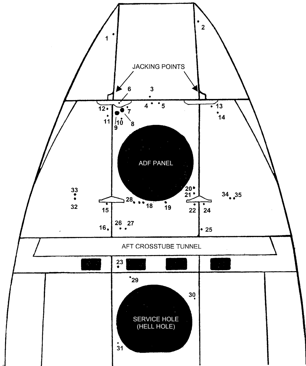
Figure 1 Model 212 Belly (Looking Up)
