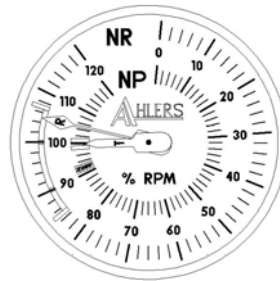
Figure 2. P/N 407-375-008-113
